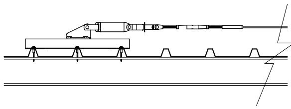
End Stanchion Assembly
