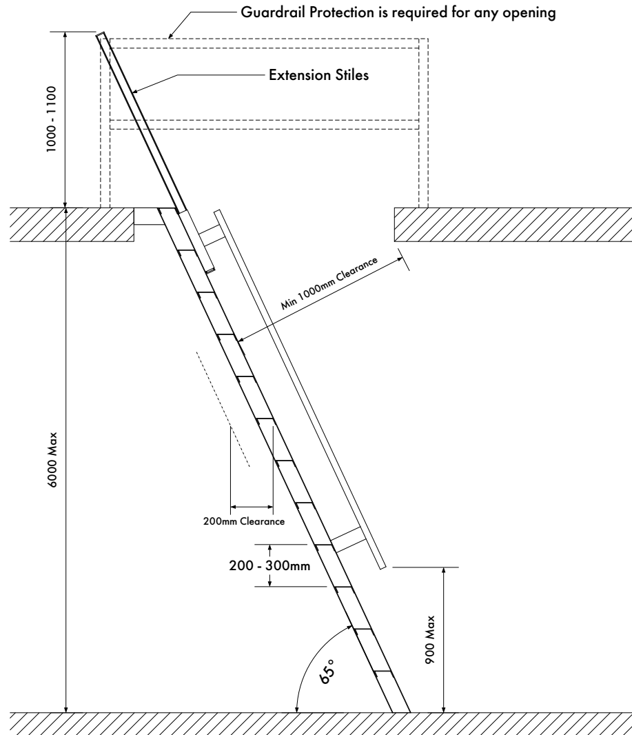
ST570 - Step Ladder for access under roof hatches
