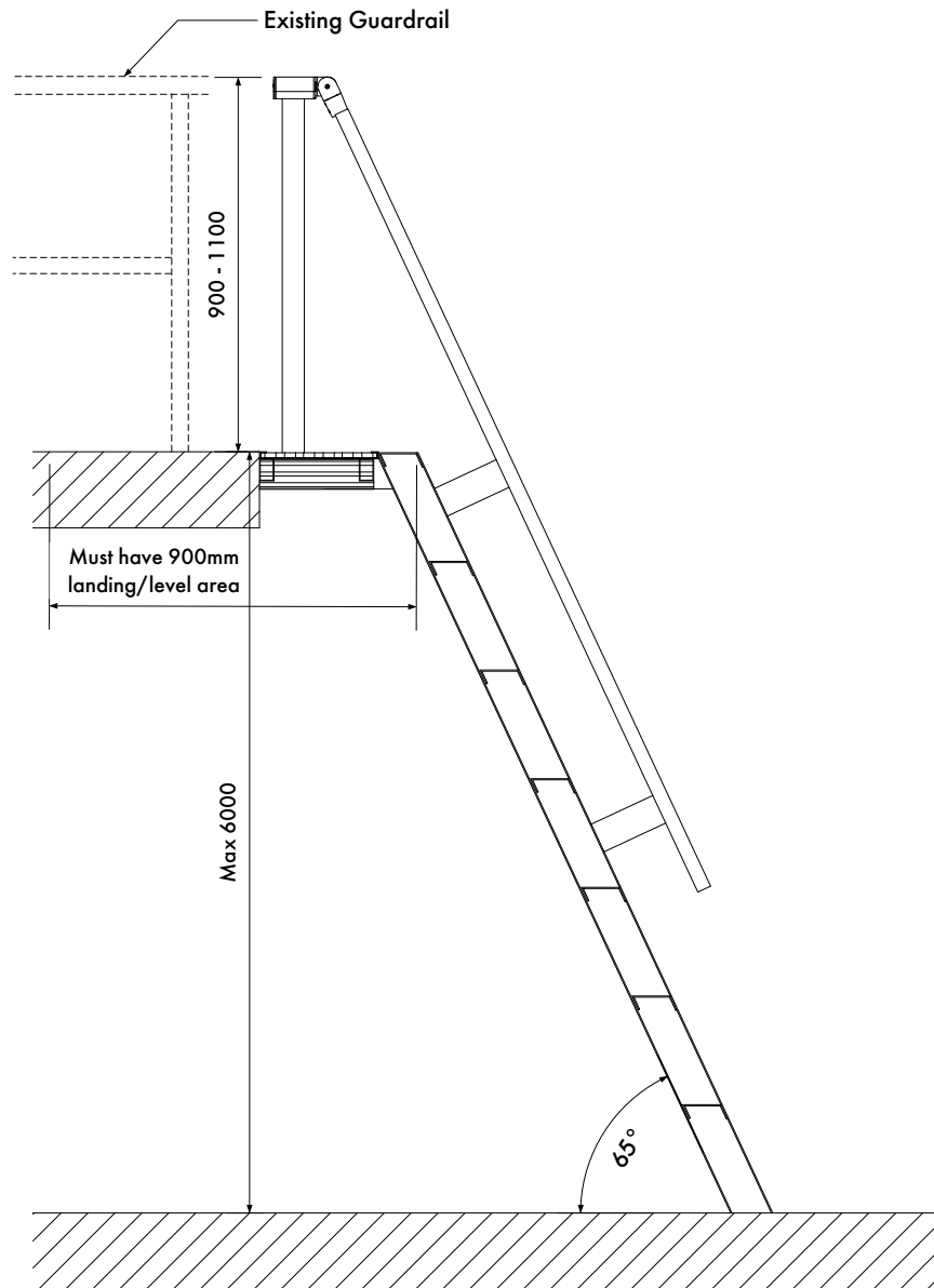
ST575 - Step Ladder for access up to an existing platform/roof (300mm landing)
