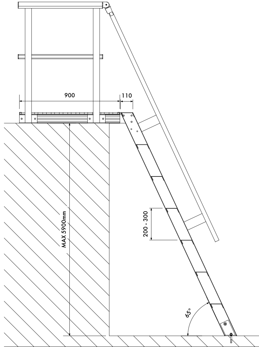
ST580 - Step Ladder for access on to an existing platform/roof (900mm landing)
