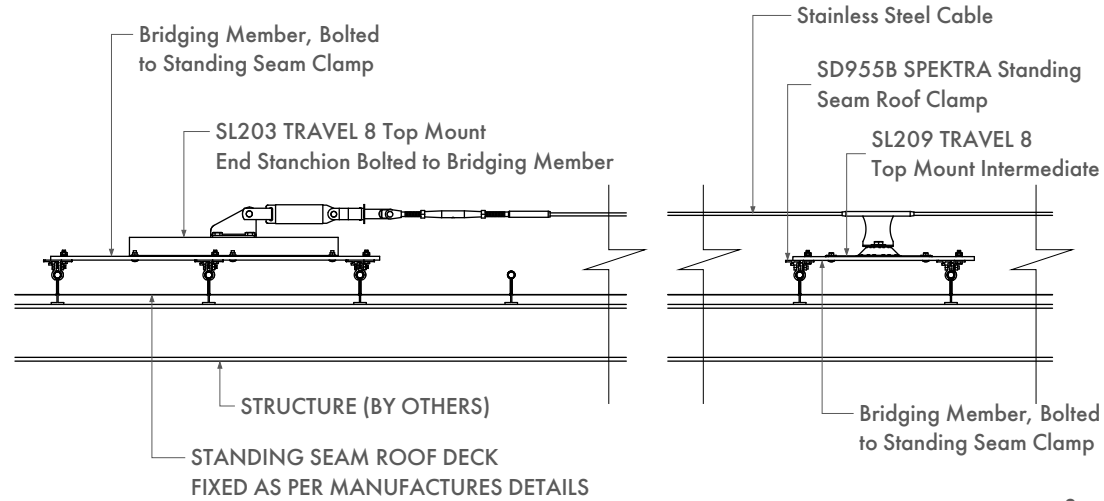
Standing Seam Roof Deck (E.g. Kingzip SF400, Kalzip 65/400, Bemo 65/400)
