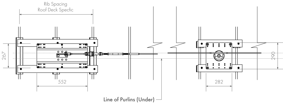
Standing Seam Roof Deck (E.g. Kingzip SF400, Kalzip 65/400, Bemo 65/400)
